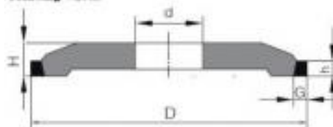
Grinding wheel:
